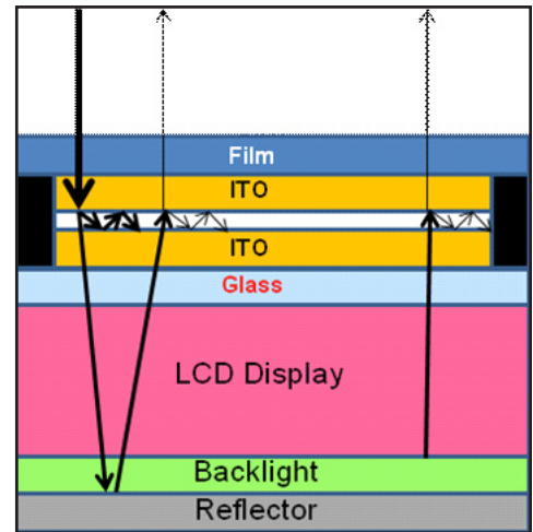
Resistive Touch Screen Construction
